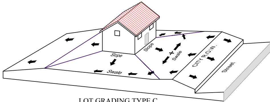
LOT GRADING TYPE C Drainage Directed Toward Rear of Lot
