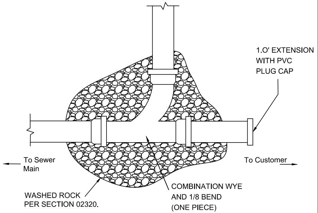
SECTION B-B
